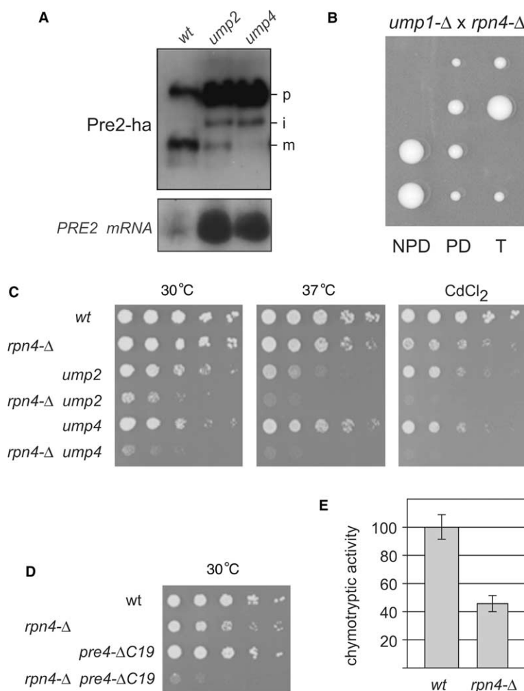
Fig. 2. Up-regulation of proteasome levels in ump mutants requires Rpn4. A : Elevated levels of \beta 5 /Pre2 were detected in crude extracts from ump2 and ump4 strains expressing Pre2-ha by anti-ha Western blotting (upper panel). p, Pro \beta 5 precursor; i, incompletely processed \beta 5 ; m, mature \beta 5 . The lower panel shows the detection of increased PRE2 transcript levels in the same mutants by Northern blotting. B : rpn4-Δ and ump1-Δ are synthetically lethal. Tetrads of strain ML3 ( ump1-Δ::HIS3 × rpn4-Δ::LEU2 ) were dissected on YPD, and viable spore clones were analyzed for histidine and leucine prototrophy. No viable His + Leu + spore clones were obtained (not shown). NPD, non-parental ditype; PD, parental ditype; T, tetratype. C : Deletion of RPN4 in the ump2 and ump4 mutants leads to strong synthetic growth defects and hypersensitivity to stresses. Serial dilutions of cells were spotted onto plates containing YPD medium with or without 30 \mu M CdCl 2 and incubated for 2 days. D : Up-regulation of proteasome levels by Rpn4 masks the effect of the pre4-ΔC19 mutation. Serial dilutions of cells were spotted onto YPD plates and incubated for 2 days. E : RPN4 is required to maintain proteasome levels under normal growth conditions. Shown are the proteasomal chymotryptic activities in crude extracts. Values are the means of four independent measurements. S.D. are indicated.
